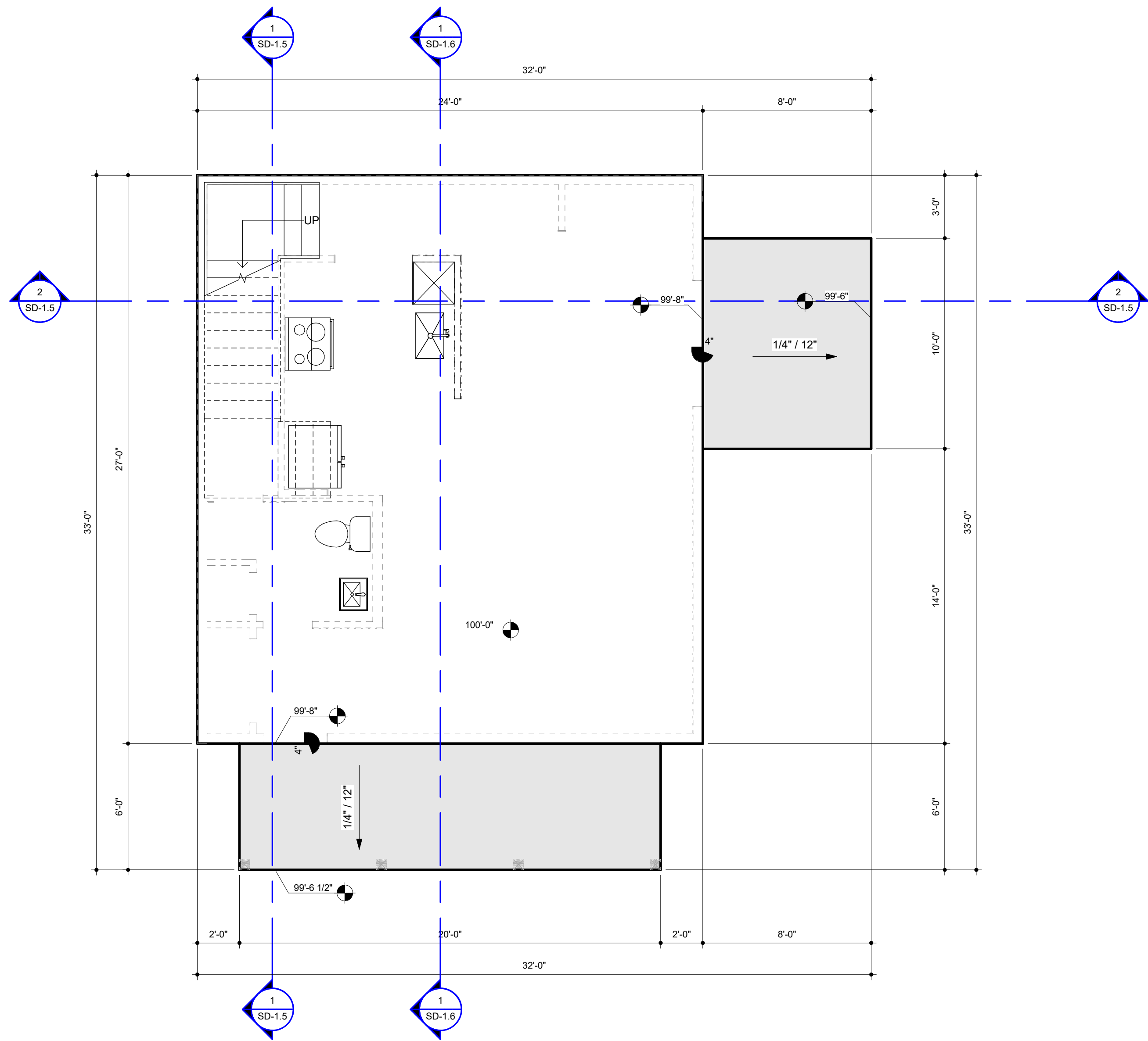
1 SD - SLAB - BUILDING 1 1/4" = 1'-0"
