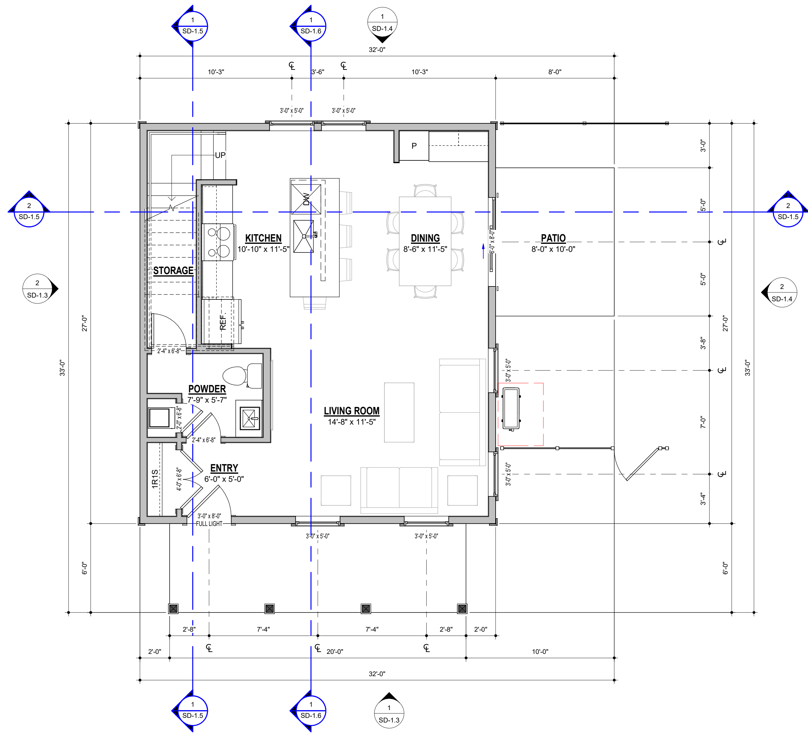
2 SD - FIRST FLOOR - BUILDING 1 1/4" = 1'-0"
