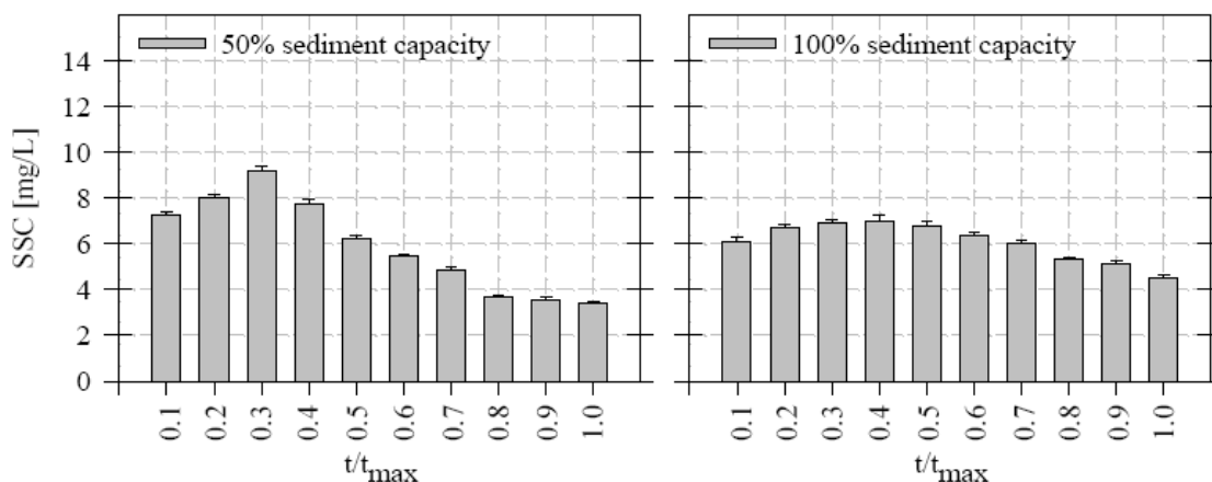
Figure 2 Individual SSC for NJDEP under 50%/100% pre-loaded sediment in STC450i as a function of time normalized to maximum run duration (10 minutes).
