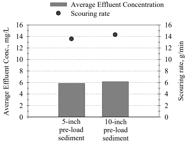
Figure 3 Scour test results for the STC450i at 565 % of MTFR (718 gpm) at 5-inch and 10-inch of NJPSD sediment pre-loaded conditions.
